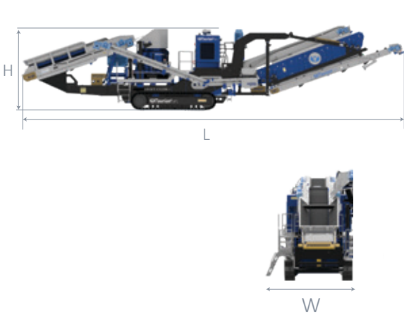
Transport Dimensions
