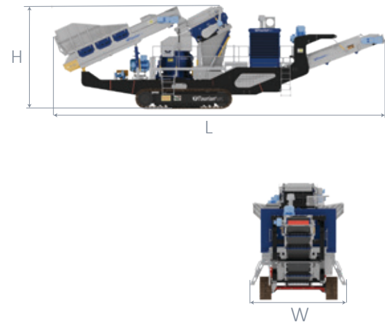
Working Dimensions
